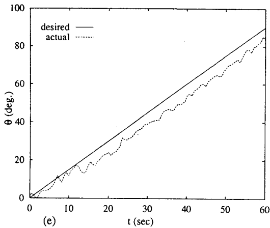
Figure 7: Visual Tracking experiment: moving electric socket. (a) Image Window. (b) Parametric eigenspace representation. Desired and actual coordinates: (c) x(t) ; (d) y(t) ; and (e) q(t) . (f) Tracking distance error d(t) .
