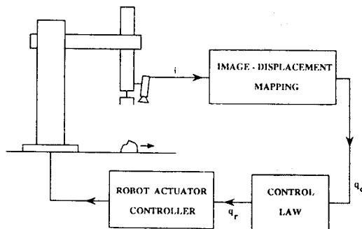
Figure 4: Schematic diagram of the visual tracking system.
