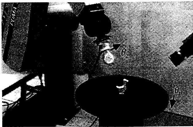
Figure 1: Setup used for automatic acquisition of object image sets. The object is placed on a motorized turntable.
