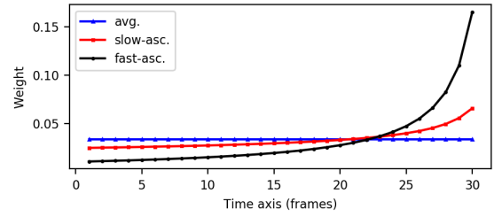
Fig. 3: Voting scheme in relation to time axis, e.g. a vehicle left-turning sequence in 30 frames.
